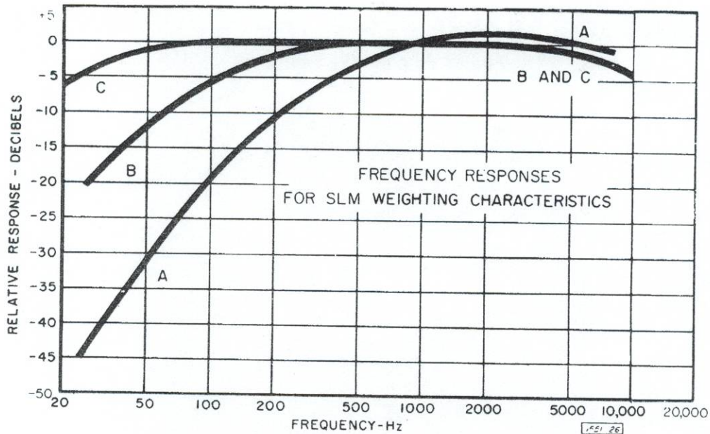
Figure 1-22. Frequency-response characteristics.
