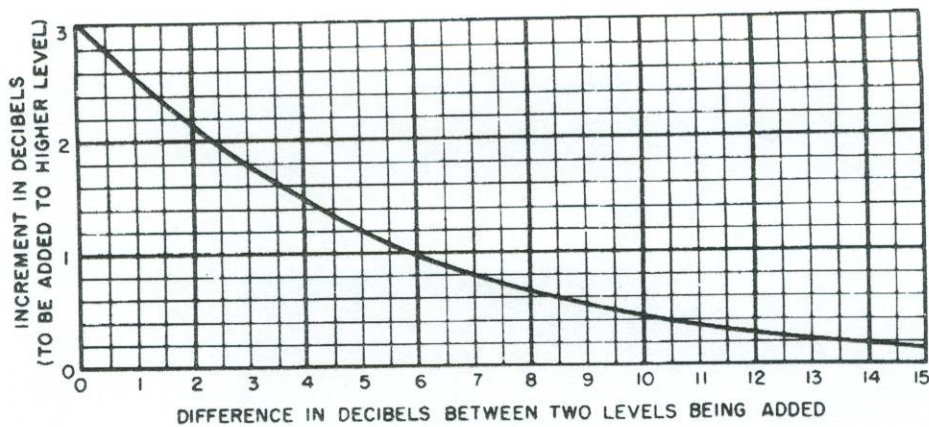
Figure 1-24. Decibel Manipulation Graph
